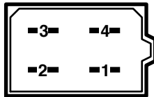
Tyco Fastin-Faston Connector
